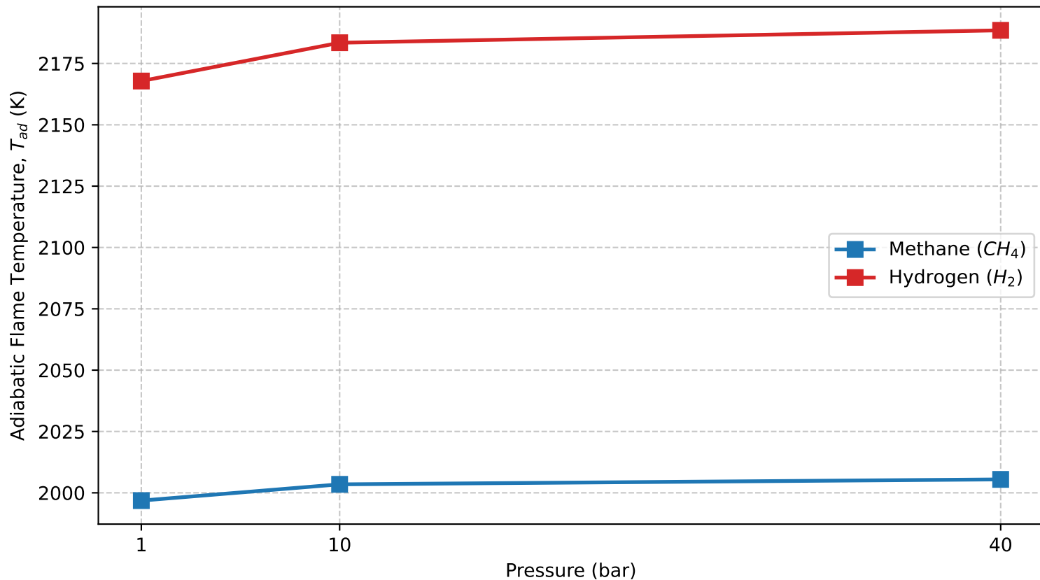
b) Adiabatic Flame Temp vs Pressure (Baseline: \phi=0.8 , T_{in}=300\text{K} )
